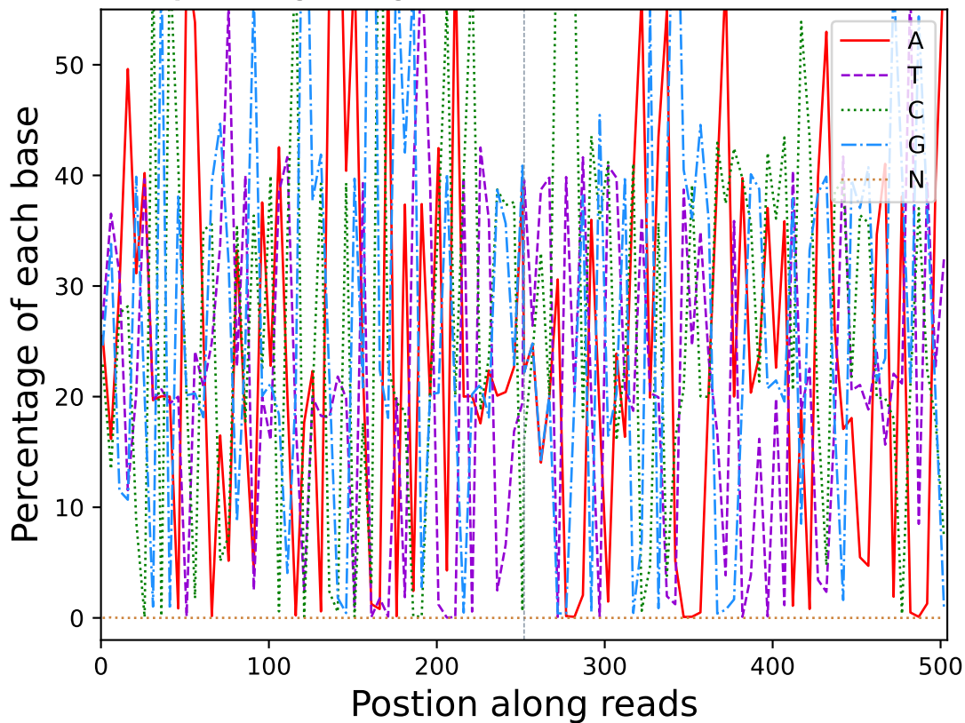
Base percentage along reads (R10119)
